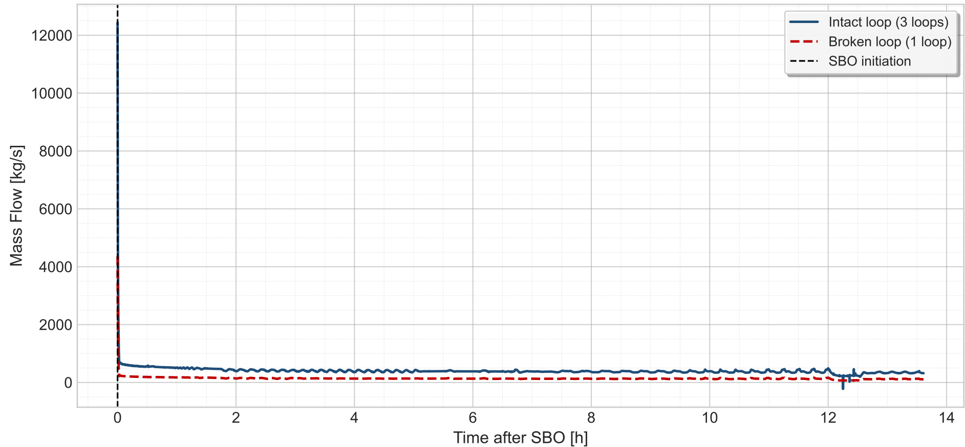
Base Case - Primary Loop Flow (Natural Circulation)
